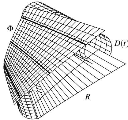
Figure 16: Envelope of a one-parameter family of congruent cylinders of revolution
