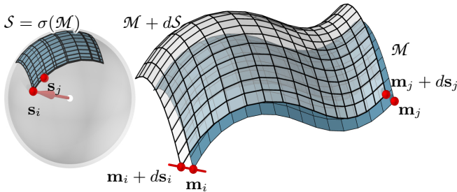
Figure 12: This figure illustrates how we assign a geometric support structure to a given mesh \mathcal{M} and thus make it buildable with optimized nodes and controlled beam heights. Optimization in the space \mathcal{P}(\mathcal{M}) yields a parallel mesh S approximating the unit sphere S^2 , thus defining offsets \mathcal{M}' = \mathcal{M} + dS at approximately constant distance d . Here S has an overfolding due to a change in the sign of curvature in \mathcal{M} , and is contained in the layer between radii 0.98 and 1.04.
