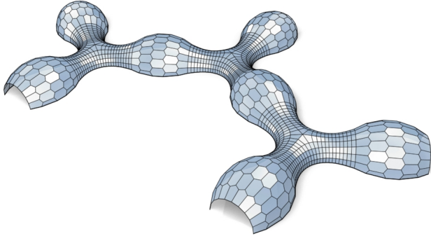
Figure 19: This design with convex faces is composed from pieces of discrete cmc surfaces obtained in different ways. The junction piece (quad mesh) was originally computed as a trioid (cf. [Grosse-Brauckmann and Polthier 1997; Schmitt 2004]) by the applet at [Schmitt 2003]. After combined optimization of mesh and Gauss image in order to achieve planarity of faces and H_F = \text{const.} , we arrive at a planar quad mesh which has H_F \in [0.966, 1.048] . The bulging pieces are hexagonal EO meshes whose mean curvature with respect to a previously chosen Koebe polyhedron as Gauss image is exactly constant.
