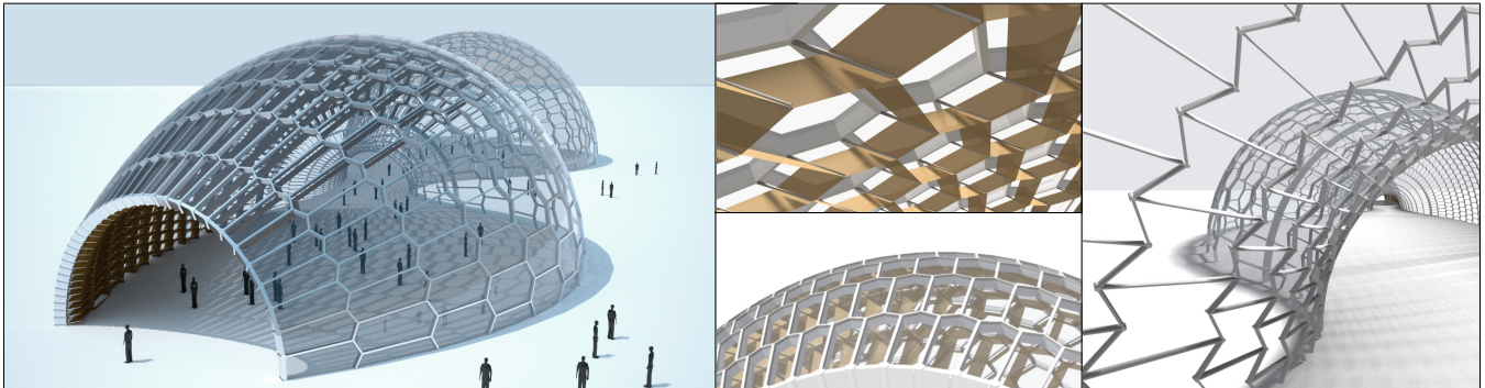
Figure 1: This architectural free form structure – built of beams of constant height meeting in optimized nodes and covered with planar glass facets – was designed using the theory and algorithms presented in this paper. Our method also allows for the construction of secondary parallel offsets at a variable distance, here physically realized as a structure designed to cast shadows which is optimized to reduce heat load for particular sun positions.
