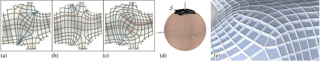
Figure 14: Meshing and construction of a support structure with optimized nodes for a given architectural freeform design. (a)–(c). A study of different conjugate curve networks is performed. We lay out a quad mesh \mathcal{M} along the network in (c) and use the method of [Liu et al. 2006] to optimize \mathcal{M} such that its faces become planar. \mathcal{M} is shown in subfigure (e). (d) We recompute a Gauss image S of \mathcal{M} which approximates the unit sphere S^2 . (e) S leads to a support structure with optimized nodes and approximately equal beam heights for \mathcal{M} .
