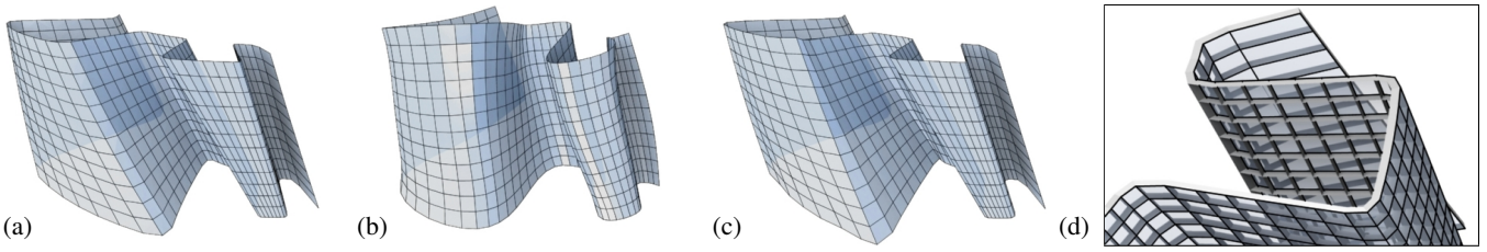
Figure 13: This figure illustrates that finding a support structure according to the method of Section 4.2 can be done with little change in the original mesh. (a) a mesh \mathcal{M} created by subdivision. (b) In order to create a geometric support structure with nice offset properties, we first follow [Liu et al. 2006] and make the mesh conical by perturbing vertices. As the intersection angles of mesh polylines in \mathcal{M} are far from 90 degrees, the optimized mesh deviates much from \mathcal{M} . (c) If \mathcal{M} is optimized to become planar, not necessarily conical, the deviations from the original mesh are small. (d) We apply our procedure for creating a support structure with approximately constant beam heights.
