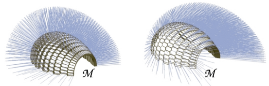
Figure 15: These two systems of ‘approximate normal vectors’ of a mesh \mathcal{M} are defined by a Gauss image S , whose edges are tangent to S^2 (left image), and the Gauss image S + \mathbf{x} (right image). They correspond to the two different support structures employed in Fig. 1.
