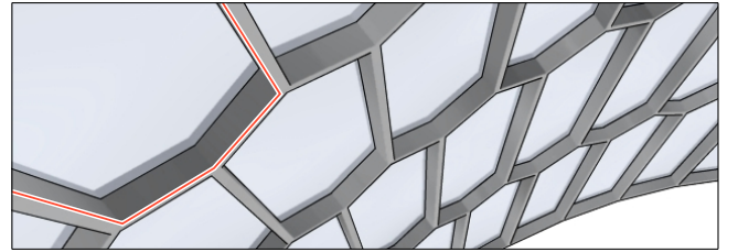
Figure 6: This construction (a detail of Fig. 1) is based on an edge offset mesh and has beams of constant height. In the positively curved areas, edges (red) of beams with rectangular cross-section have an exact intersection at the nodes, which follows from Prop. 3.
