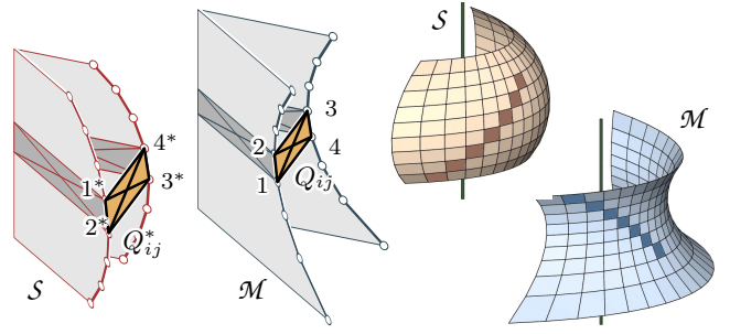
Figure 17: Construction of simple minimal quad meshes via parallelism of diagonals. The meshes \mathcal{M}, \mathcal{S} carry ‘horizontal’ polylines in horizontal planes and ‘meridian polylines’ in planes through a fixed axis. \mathcal{S}, \mathcal{M} are parallel – note corresponding faces Q_{ij} and Q_{ij}^* – but the correspondence is orientation-reversing. The mean curvature of the face Q_{ij} in the mesh \mathcal{M} with respect to the Gauss image \mathcal{S} vanishes if and only if diagonals in Q_{ij} are parallel to diagonals in Q_{ij}^* ( 13 \parallel 2^*4^* and 24 \parallel 1^*3^* ).
