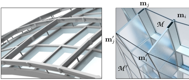
Figure 2: Multi-layer constructions based on the geometric support structure defined by two parallel meshes \mathcal{M} , \mathcal{M}' at approximately constant distance. On the left, the lower layer of the glass roof is suspended from the upper layer which has a structural function. The right hand image shows a rudimentary construction of a glass facade where the closed space between layers has an insulating function.
