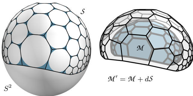
Figure 8: A mesh \mathcal{M} with an edge offset mesh \mathcal{M}' at distance d has a parallel mesh S = (\mathcal{M}' - \mathcal{M})/d whose edges are tangent to the unit sphere S^2 . The faces of S intersect S^2 in a circle packing, cf. Section 3.2.
