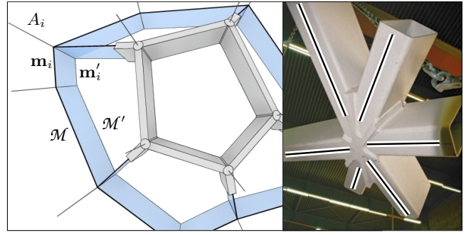
Figure 4: Left: This figure shows nodes, supporting beams, and the underlying geometric support structure of a steel/glass construction, based on a mesh \mathcal{M} (vertices \mathbf{m}_i ) and its parallel mesh \mathcal{M}' (vertices \mathbf{m}'_i ). All beams are symmetric with respect to their central plane (blue); at an optimized ( torsion-free ) node \mathbf{m}_i the central planes of supporting beams pass through the node axis A_i = \mathbf{m}_i \vee \mathbf{m}'_i . Right: A node without axis, with geometric torsion.
