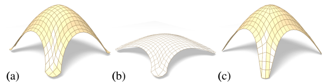
Figure 12: Directly enforcing planarity of the faces of even a very simple self-supporting quad-mesh vault (a) results in a surface far removed from the original design (b). Starting instead from a remeshing of the surface with edges following relative principal curvature directions yields a self-supporting, PQ mesh far more faithful to the original (c).
