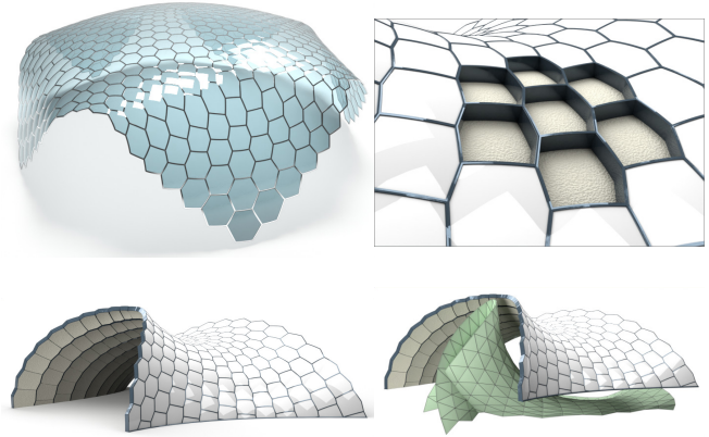
Fig. 32. SHex-meshes with support structures from intersecting tangential spheres. Top-Left: An SHex-mesh paneling with visually convex hexagons. However note that these hexagons are not planar and the classical notion of convexity does not apply here. Bottom-Left: An SHex-mesh paneling a negatively curved surface. Again, the spherical hexagonal faces give the impression of convex hexagons which is only possible because the faces are proper spheres. Planar faces paneling a negatively curved region would result in bow-tie shaped hexagons. Top-Right: These meshes possess a geometric support structure as illustrated on a detail of the bottom-left SHex-mesh. Bottom-Right: The vertices of the green mesh are the centers of the spheres. Note that the combinatorics of the mesh of centers which is the same as the combinatorics of the mesh of spheres in P^4 is dual to the sphere mesh.
