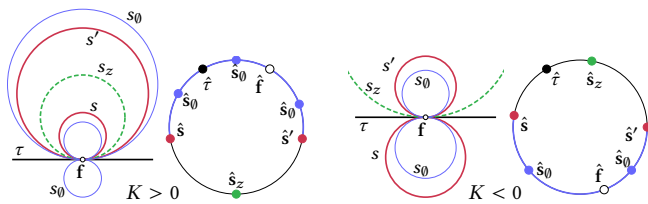
Fig. 31. The parabolic pencil of tangent spheres contains the surface point f , the tangent plane \tau , the two curvature spheres s, s' (red), and the central sphere s_z (green). In the projective model of Möbius geometry the sphere pencil is represented by the points of a projective line which is topologically a circle, split into two segments by the curvature spheres. On this circle \hat{s}_z and \hat{f} lie in different segments. The spheres s_0 of the pencil which locally do not intersect the surface (blue) lie in the same segment as the point.
