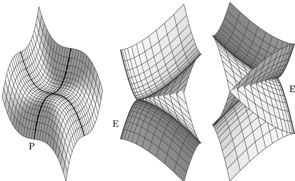
Fig. 2. Graph surface (left) of a cubic polynomial and the associated LN surface (center and right).
