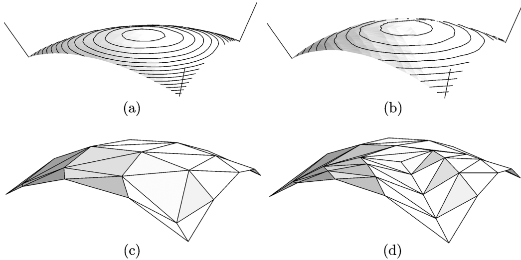
Fig. 3. LN surfaces interpolating three points with associated normal vectors (a), (b) and their control nets (c), (d). The surfaces have been generated using singularly parameterized surfaces (a), (c) and Clough–Tocher splits (b), (d).
