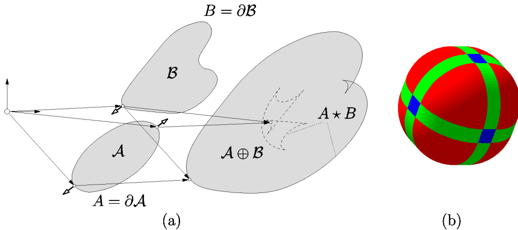
Fig. 1. (a) Minkowski sum of two planar domains and the convolution of their boundaries. (b) Minkowski sum of a ball and a cube.
